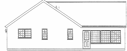
North West Elevation
